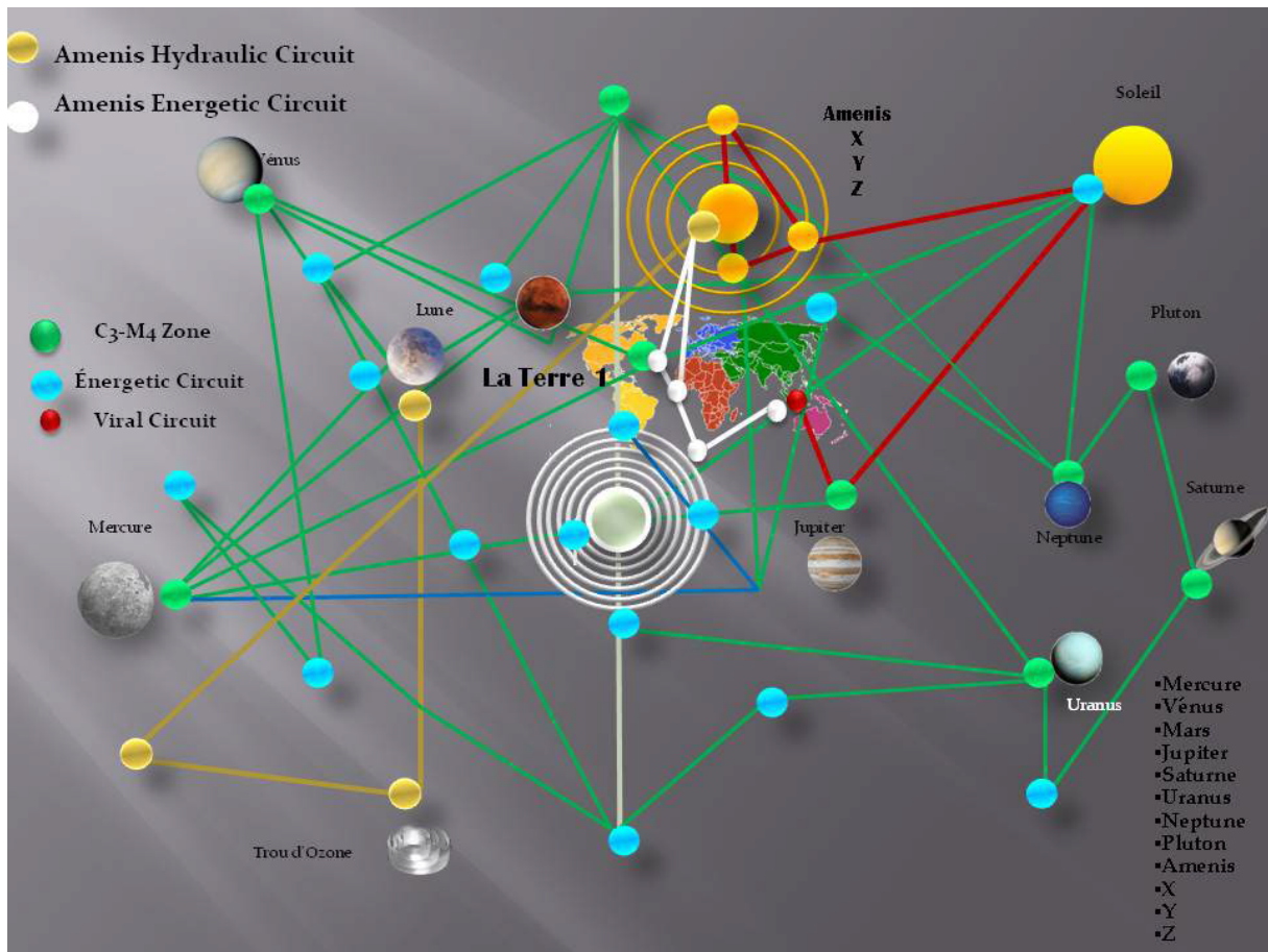
Figure 1: Interplanetary solar system.
